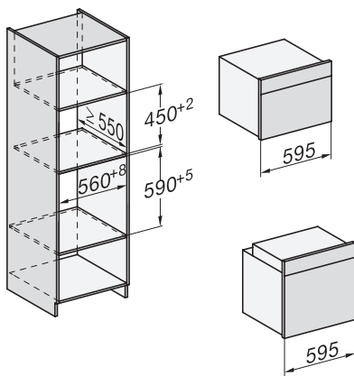
H226x-1B/BP/E/EP/I/P, H2760B/BP, H28x0B/BP, H7x40BM/BMX, H7x6x8/BP/BPX, installation drawings
